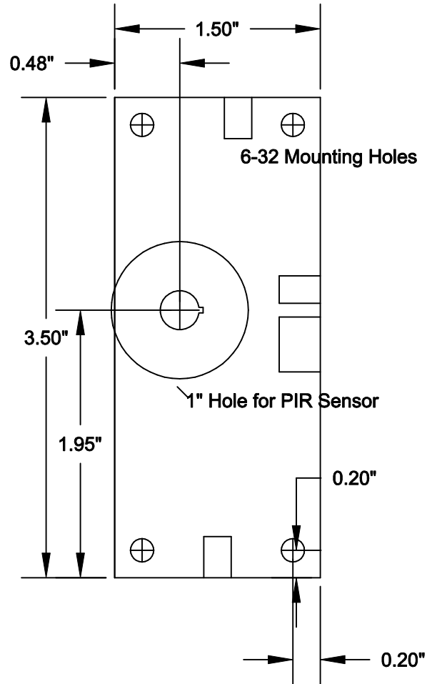
YetiCam Version 1.3 Vertical Mounting Bottom View
