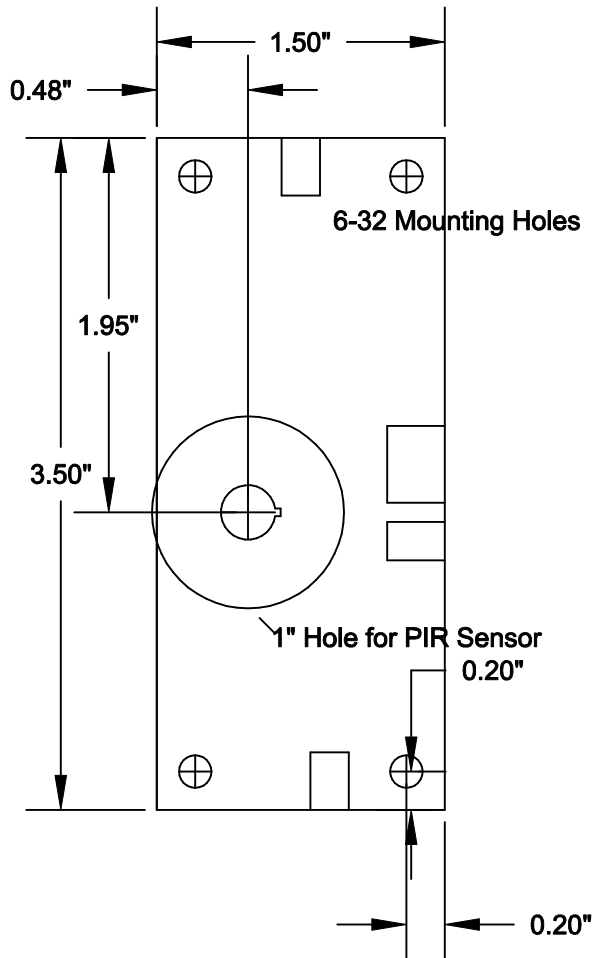
YetiCam Version 1.3 Vertical Mounting Top View
